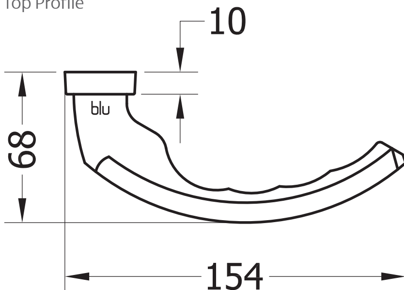
Top Profile
